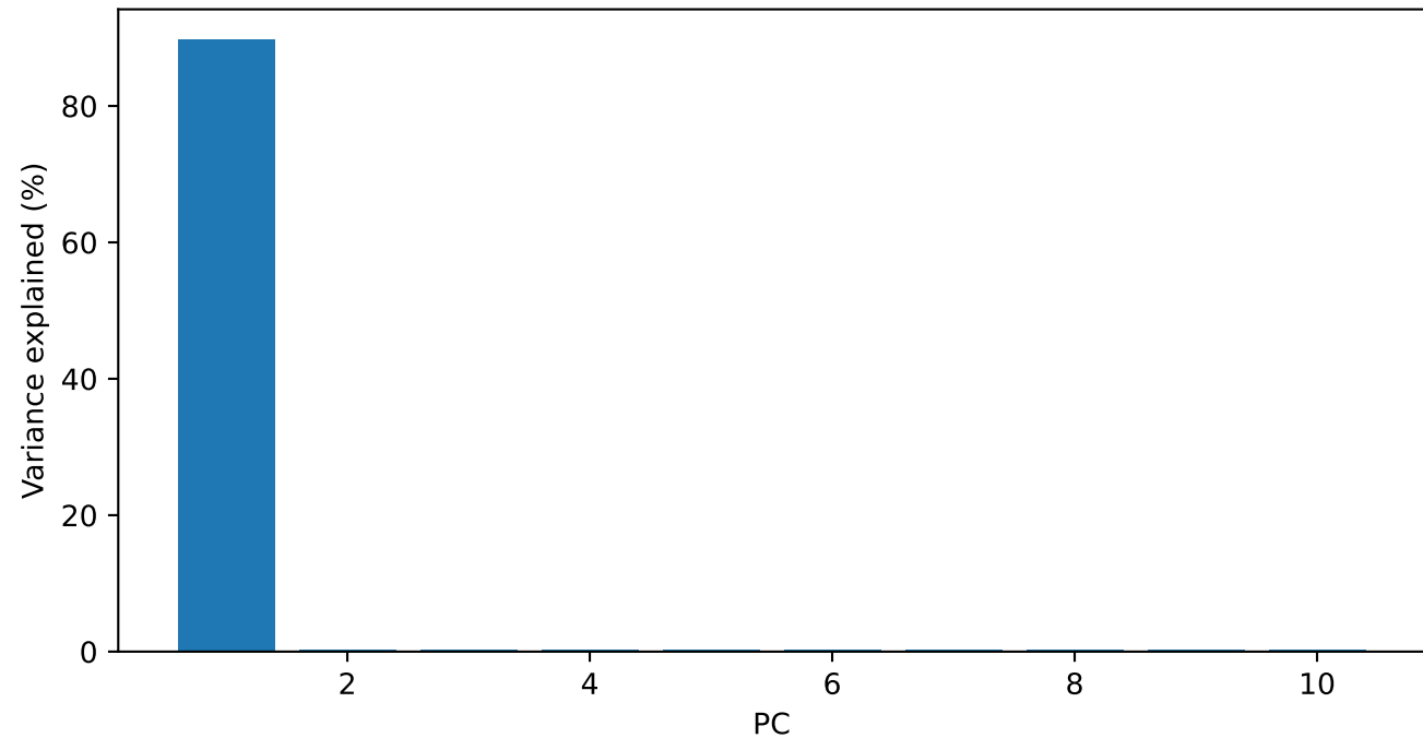
PCA (expression): variance explained
